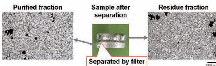
Impurity element removal method in melting and solidification process.
