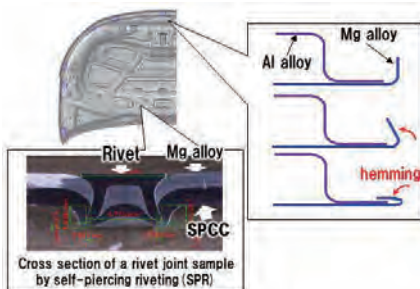
Development of Mg alloys with excellent plastic workability for mechanical fastening.
