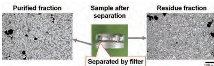
Impurity element removal method in melting and solidification process.
