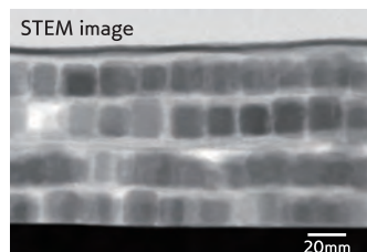
← Graphene ← BaTiO 3 ← Graphene ← BaTiO 3 ← Graphene ← BaTiO 3 ← Graphene ← BaTiO 3 ← Platinum electrode
