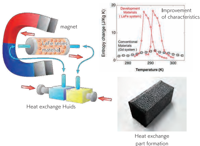
Development and modeling of magnetic refrigeration materials
